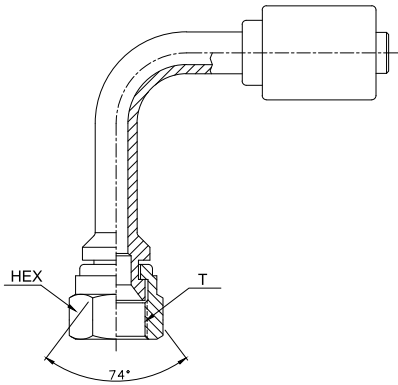
JIC SWIVEL FEMALE 74° CONE SEAT LONG DROP 90° SWEPT ELBOW:RNJ9-L
