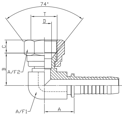
JIC SWIVEL FEMALE 74° CONE SEAT 90° COMPACT ELBOW:NJC9
