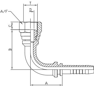
FRENCH METRIC SWIVEL FEMALE 90° ELBOW GAZ TYPE:NMG9
