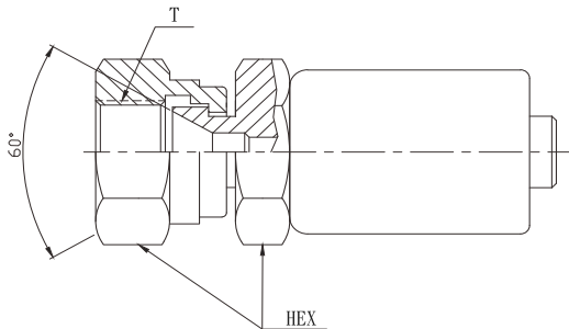
METRIC SWIVEL FEMALE 60° CONE SEAT:RNMK
