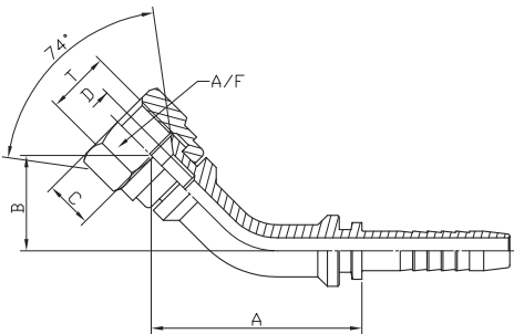
JIC SWIVEL FEMALE 74° CONE SEAT 45° SWEPT ELBOW: NJ4
