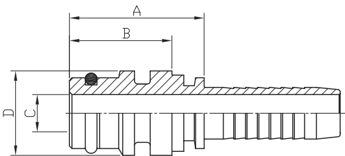
SAE STAPLE-LOCK MALE:SLOK
