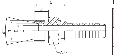
FRENCH METRIC MALE 24° CONE SEAT MILLIMETRIC TYPE:MMI
