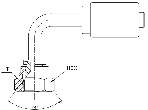
JIC SWIVEL FEMALE 74° CONE SEAT 90° SWEPT ELBOW:RNJ9
