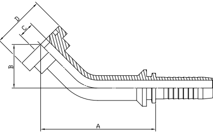
SAE FLANGE 45° SWEPT ELBOW SERIES CODE 62:PH4
