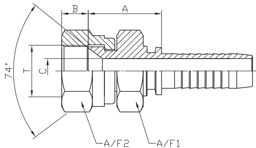
JIC SWIVEL FEMALE 74° CONE SEAT DOUBLE HEX:NJH
