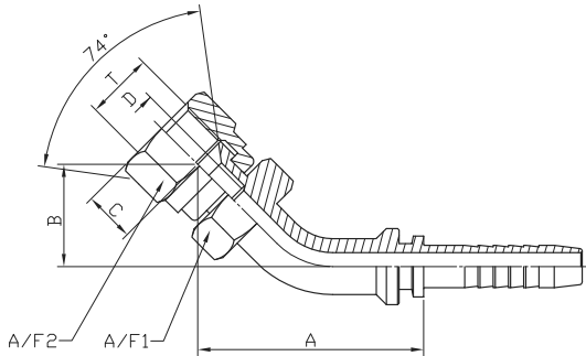
JIC SWIVEL FEMALE 74° CONE SEAT DOUBLE HEX 45° SWEPT ELBOW:NJH4
