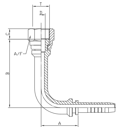
ORFS SWIVEL FEMALE 90° LONG DROP SWEPT ELBOW:NOR9-L
