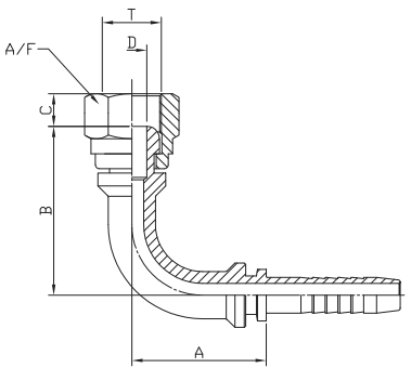
METRIC MULTISEAL SWIVEL FEMALE LIGHT DUTY 90° ELBOW:NMML9
