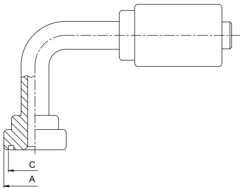
SAE FLANGE 90°SWEPT ELBOW CODE 62:RPH9
