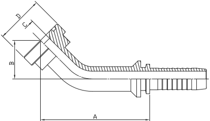
FLANGE 45° ELBOW KOMATSU:PAJK4
