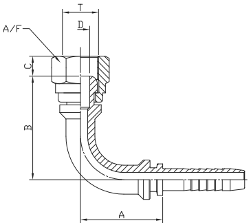
METRIC MULTISEAL SWIVEL FEMALE HEAVY DUTY 90° ELBOW:NMMH9
