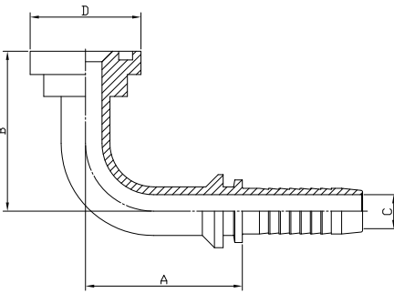
SAE FLANGE 90° SWEPT ELBOW SERIES CODE 62:PH9
