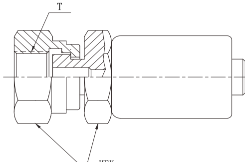
BSP SWIVEL FEMALE FLAT FACED:RNUF
