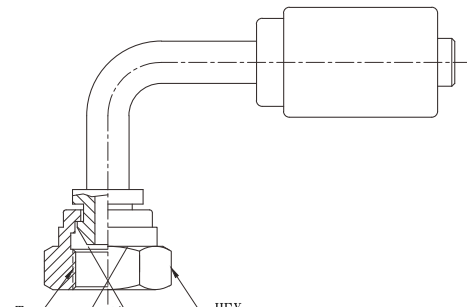
BSP SWIVEL FEMALE 60° CONE 90° SWEPT ELBOW:RNU9
