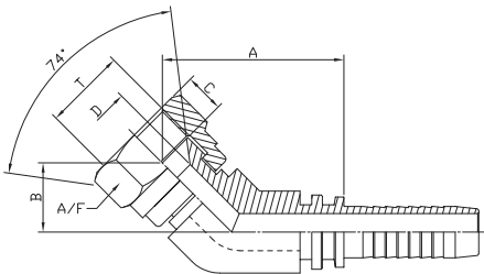
JIC SWIVEL FEMALE 74° CONE SEAT 45° COMPACT ELBOW: NJC4
