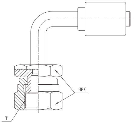
ORFS SWIVEL FEMALE FLAT FACED 90° ELBOW:RNOR9
