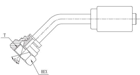
BSP SWIVEL FEMALE 60° CONE 45° SWEPT ELBOW:RNU4
