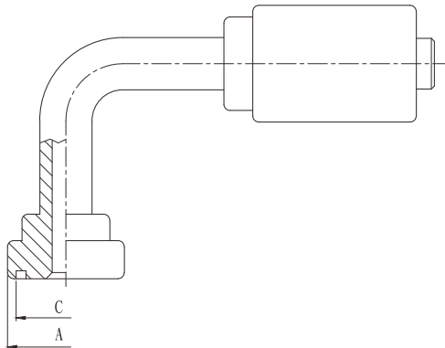
SAE FLANGE 90° SWEPT ELBOWCODE 61: RPA9
