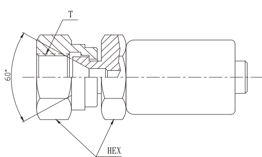
BSP SWIVEL FEMALE 60° CONE SEAT:RNUK
