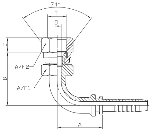
JIC SWIVEL FEMALE 74° CONE SEAT DOUBLE HEX 90° SWEPT ELBOW:NJH9
