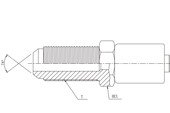
JIC MALE 74° CONE BULKHEAD:RMJB
