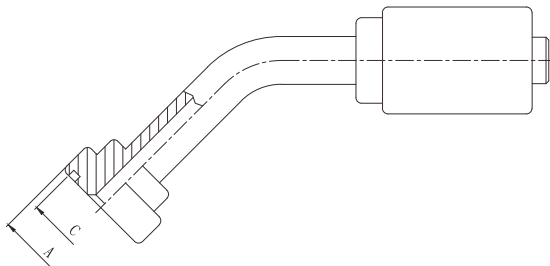
SAE FLANGE 45° SWEPT ELBOWCODE 61: RPA4
