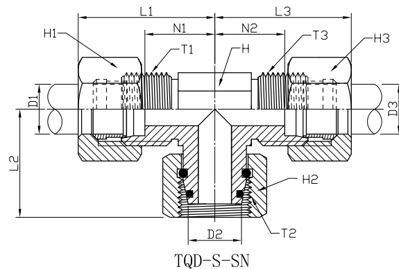
METRIC MALE 24° X METRIC SWIVEL FEMALE O-RING BRANCH X METRIC MALE 24° RUN TEE LIGHT DUTY: TQD-S / TQD-S-SN
