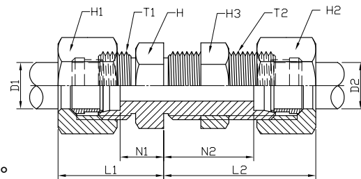
IQD-K-N-SN (LOCK NUT INCLUDED)
