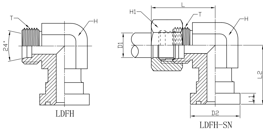
METRIC MALE 24° X SAE FLANGE 62 CODE LIGHT DUTY 90° ELBOW: LDFH / LDFH-SN
