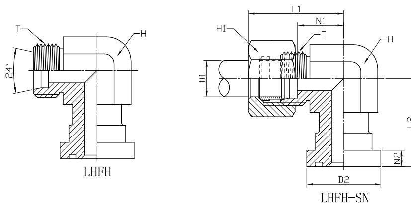
METRIC MALE 24° X SAE FLANGE 62 CODE HEAVY DUTY 90° ELBOW: LHFH / LHFH-SN
