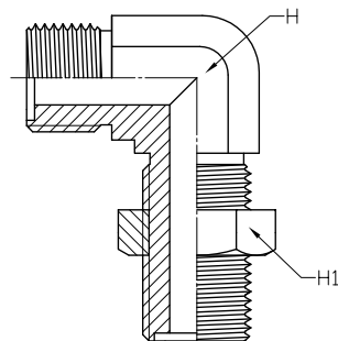
LQM-K-N (LOCK NUT INCLUDED)
