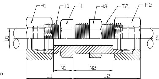
IQH-K-N-SN (LOCK NUT INCLUDED)
