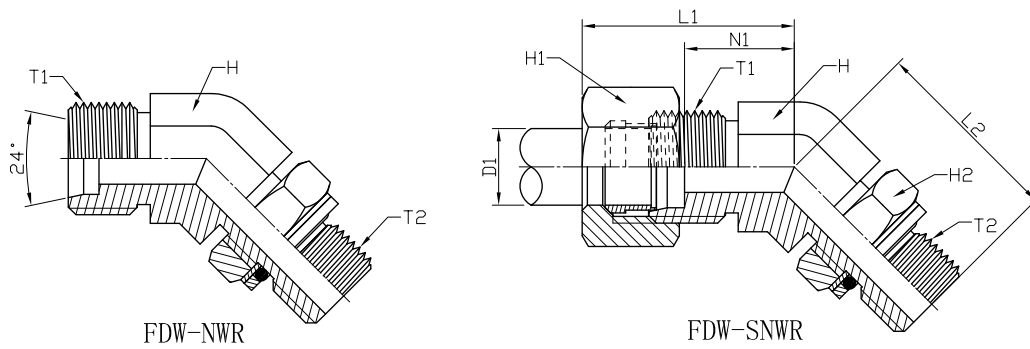
METRIC MALE 24° X METRIC MALE WITH LOCKING NUT WASHER O-RING LIGHT DUTY 45° ELBOW: FDW-NWR / FDW-SNWR
