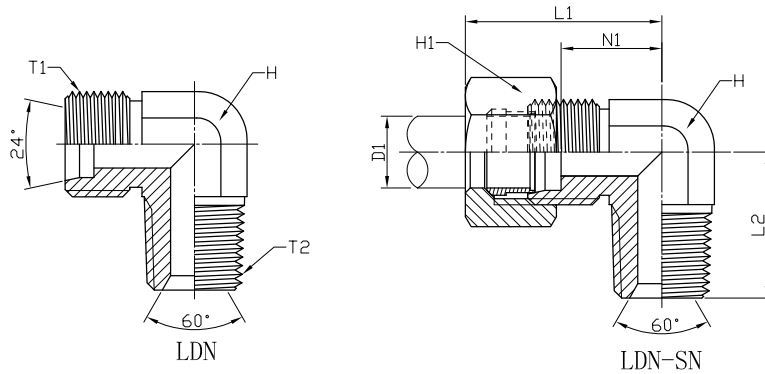
METRIC MALE 24° X NPT MALE LIGHT DUTY 90° ELBOW: LDN / LDN-SN
