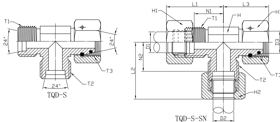
METRIC MALE 24° X METRIC MALE 24° BRANCH X METRIC SWIVEL FEMALE O-RING RUN TEE LIGHT DUTY: TQD-S / TQD-S-SN
