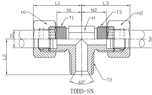
METRIC MALE 24° WITH NUT & RING X BSPT MALE BRANCH X METRIC MALE 24° WITH NUT & RING RUN TEE: TDBD-SN
