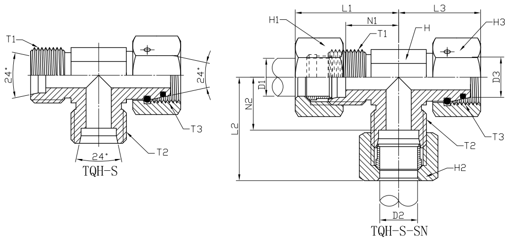
METRIC MALE 24° X METRIC MALE 24° BRANCH X METRIC SWIVEL FEMALE O-RING RUN TEE HEAVY DUTY: TQH-S / TQH-S-SN
