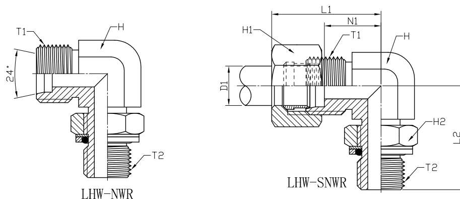
METRIC MALE 24° X METRIC MALE WITH LOCKING NUT WASHER O-RING HEAVY DUTY 90° ELBOW: LHW-NWR / LHW-SNWR
