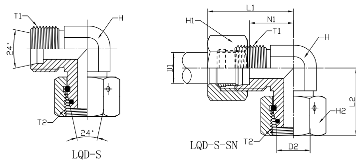
METRIC MALE 24° X METRIC SWIVEL FEMALE 24° O-RING LIGHT DUTY 90° ELBOW: LQD-S / LQD-S-SN
