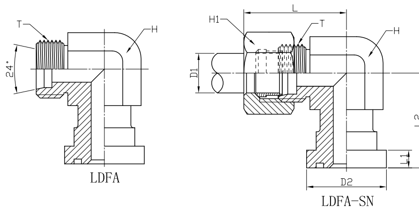
METRIC MALE 24° X SAE FLANGE 61 CODE LIGHT DUTY 90° ELBOW: LDFA / LDFA-SN
