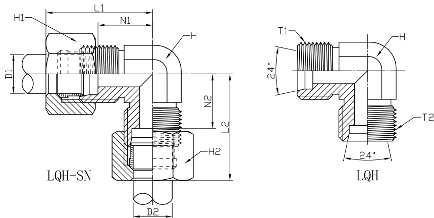
METRIC MALE 24° HEAVY DUTY 90° ELBOW: LQH / LQH-SN
