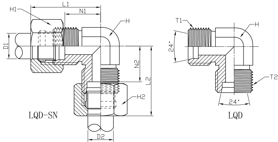
METRIC MALE 24° LIGHT DUTY 90° ELBOW: LQD / LQD-SN
