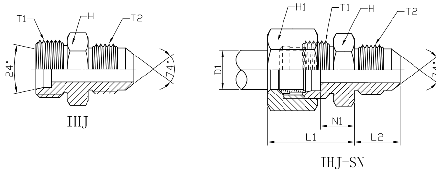
METRIC MALE 24° X JIC MALE HEAVY DUTY: IHJ / IHJ-SN
