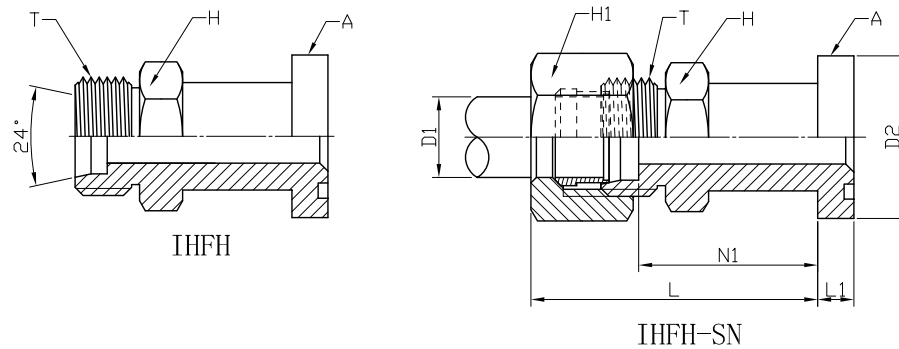
METRIC MALE 24° X SAE FLANGE 62 CODE HEAVY DUTY: IHFH / IHFH-SN
