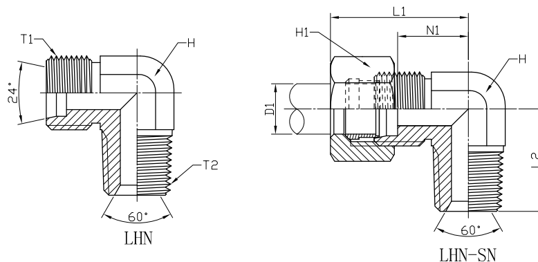
METRIC MALE 24° X NPT MALE HEAVY DUTY 90° ELBOW: LHN / LHN-SN
