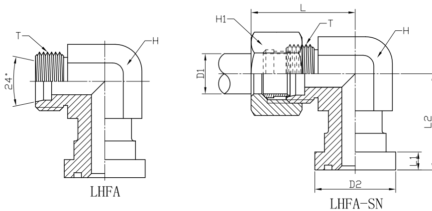
METRIC MALE 24° X SAE FLANGE 61 CODE HEAVY DUTY 90° ELBOW: LHFA / LHFA-SN
