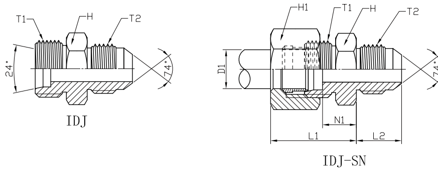
METRIC MALE 24° X JIC MALE LIGHT DUTY: IDJ / IDJ-SN
