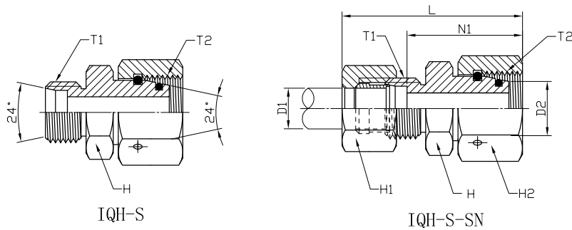
METRIC MALE 24° X METRIC SWIVEL FEMALE 24° O-RING HEAVY DUTY: IQH-S / IQH-S-SN
