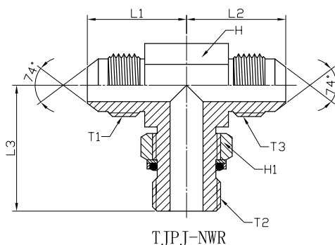
JIC MALE 74° CONE X BSP MALE WITH LOCKING NUT WASHER O-RING BRANCH X JIC MALE 74° CONE RUN TEE: TJPJ-NWR
