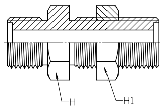
IQM-K-N (LOCK NUT INCLUDED)
