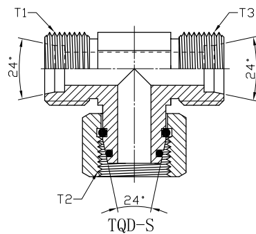
METRIC MALE 24° X METRIC SWIVEL FEMALE O-RING BRANCH X METRIC MALE 24° RUN TEE LIGHT DUTY: TQD-S / TQD-S-SN
