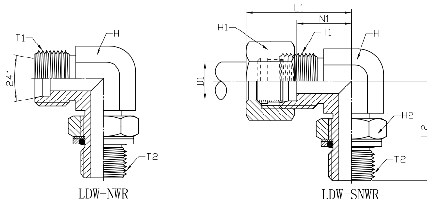
METRIC MALE 24° X METRIC MALE WITH LOCKING NUT WASHER O-RING LIGHT DUTY 90° ELBOW: LDW-NWR / LDW-SNWR
