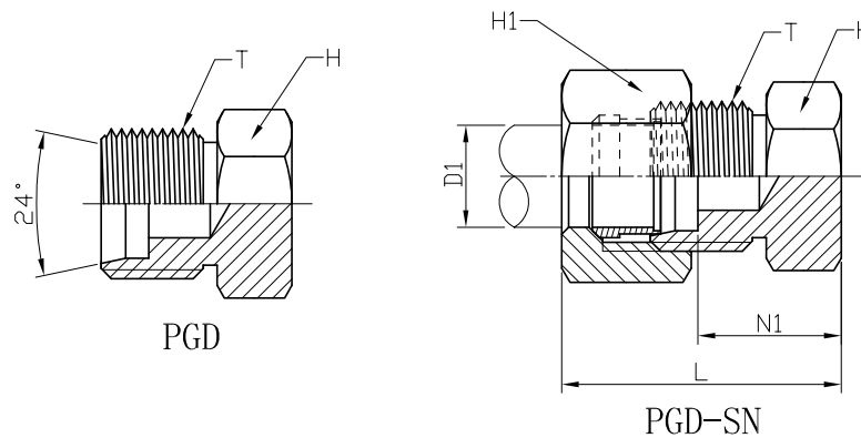
METRIC MALE 24° PLUG LIGHT DUTY: PGD / PGD-SN
