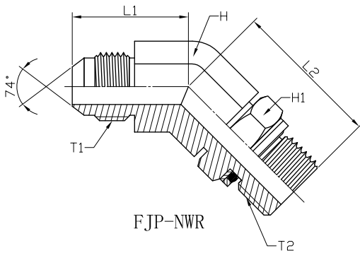
JIC MALE 74° CONE X BSP MALE WITH LOCKING NUT WASHER O-RING 45° ELBOW: FJP-NWR
