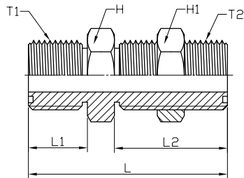
IQR-K-N (LOCK NUT INCLUDED)
