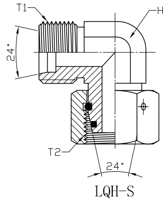
METRIC MALE 24° X METRIC SWIVEL FEMALE 24° O-RING HEAVY DUTY 90° ELBOW: LQH-S / LQH-S-SN
