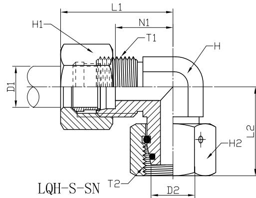
METRIC MALE 24° X METRIC SWIVEL FEMALE 24° O-RING HEAVY DUTY 90° ELBOW: LQH-S / LQH-S-SN
