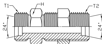
IQH-K-N (LOCK NUT INCLUDED)
