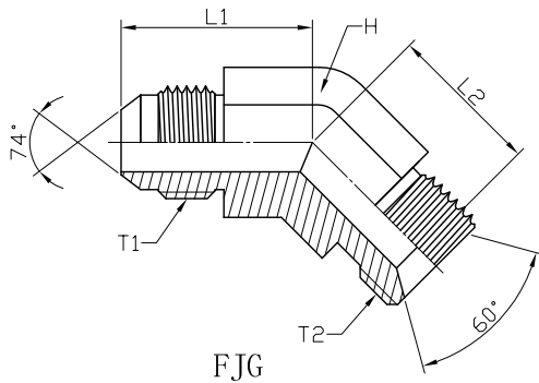
JIC MALE 74° CONE X BSP MALE 60° CONE SEAT 45° ELBOW: FJG
