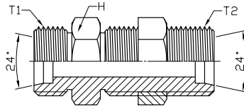
IQD-K-N (LOCK NUT INCLUDED)
