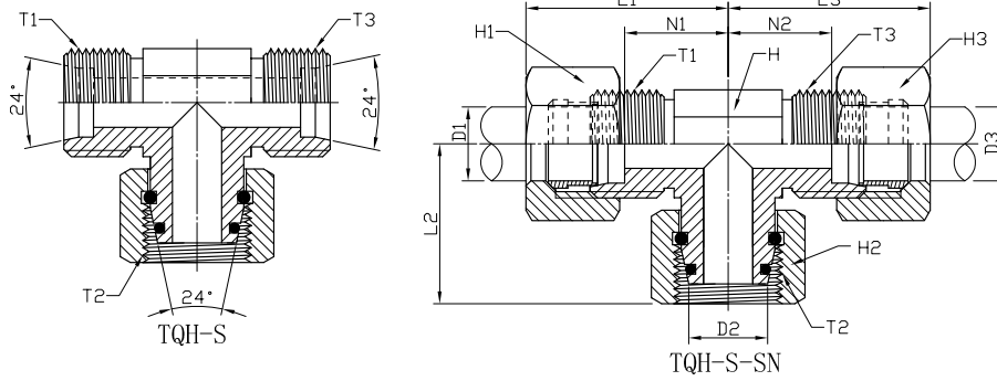
METRIC MALE 24° X METRIC SWIVEL FEMALE O-RING BRANCH X METRIC MALE 24° RUN TEE HEAVY DUTY: TQH-S / TQH-S-SN
