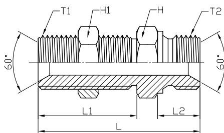
IQG-K-N (LOCK NUT INCLUDED)
