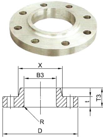
LAP JOINT
