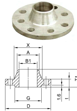
WELDING NECK
