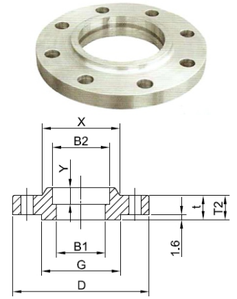
SOCKET WELDING
