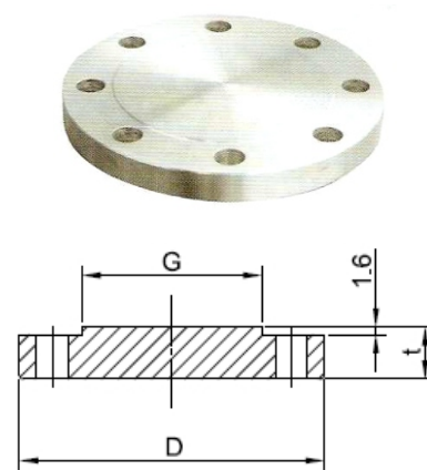
BLIND
