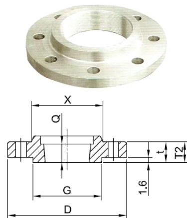
THREADED
