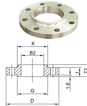
SLIP-ON
